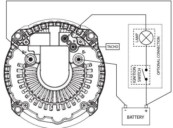
8SC Wiring Diagram
